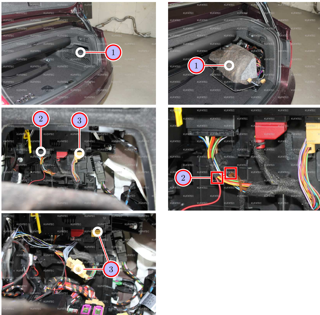
Figure 2: Connection Cabrio Comfort Module
