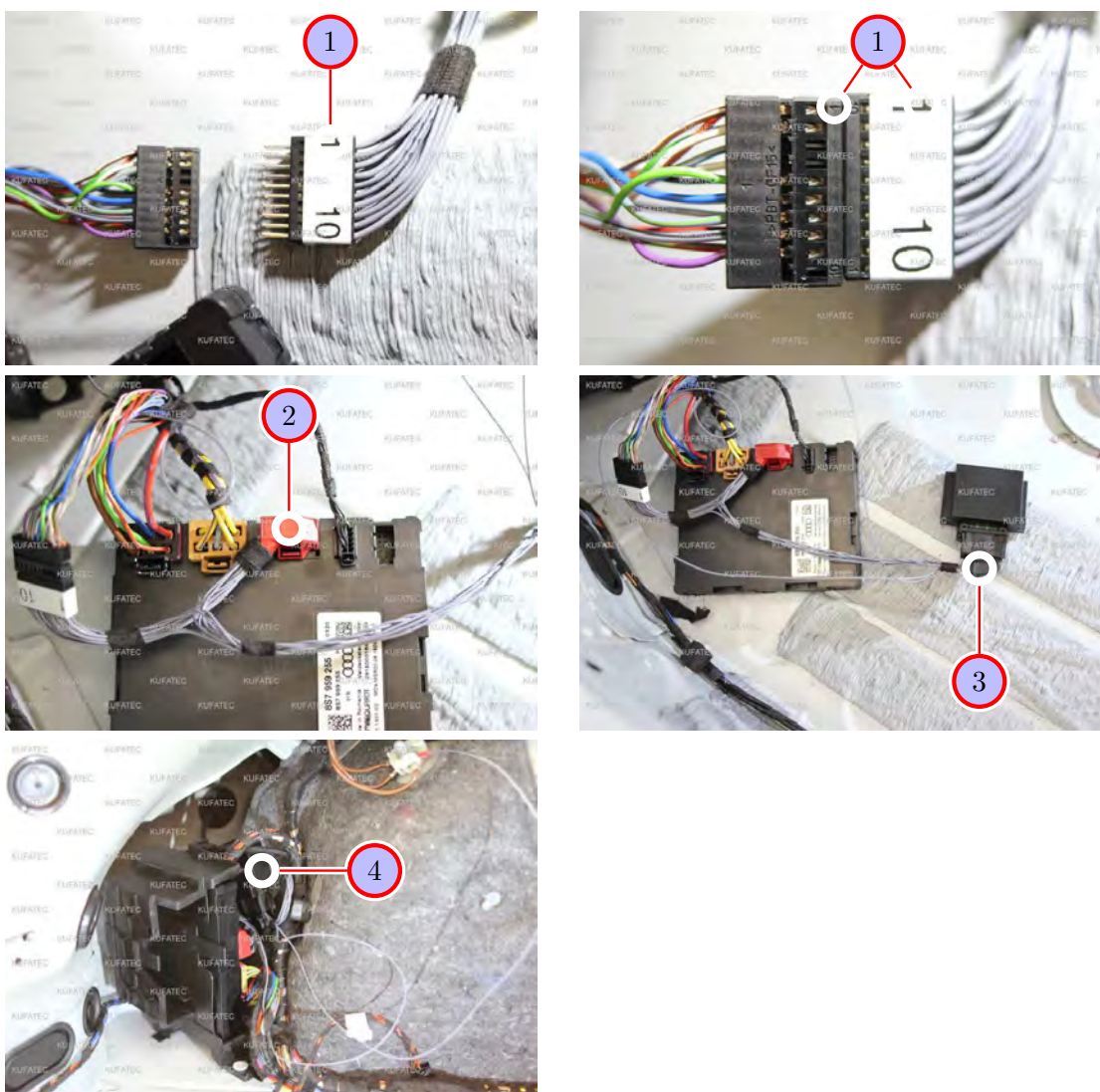
Figure 6: Connection Cabrio Pro Comfort Module
