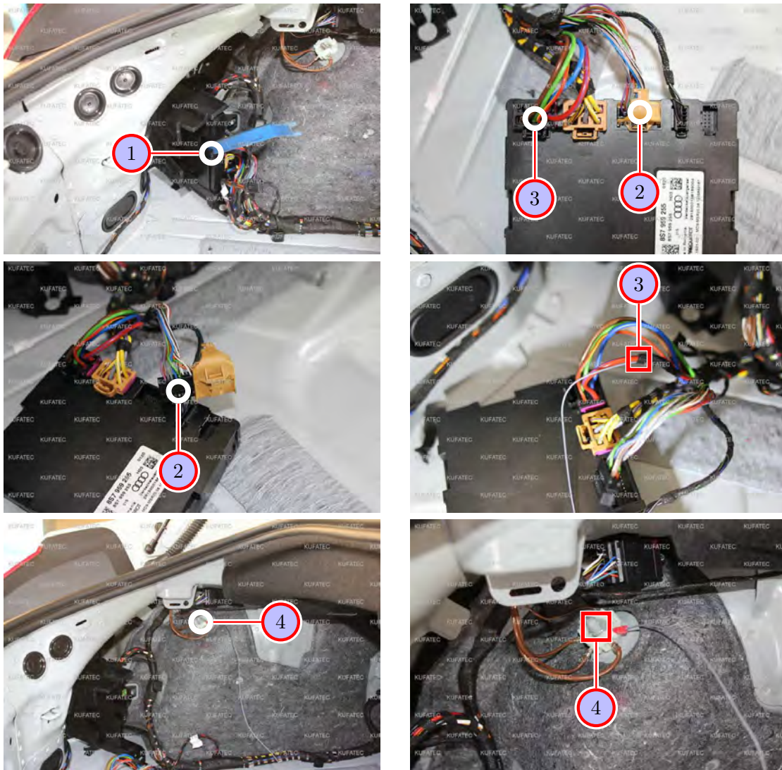
Figure 5: Connection Cabrio Pro Comfort Module
